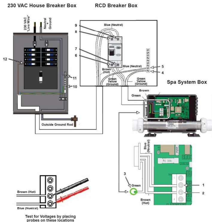
Figure 3. Wiring Schematic for 50 Hz Systems
