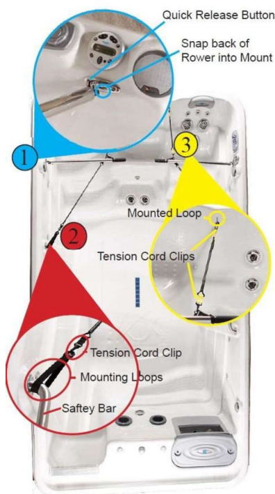
Figure 11. Rowing Equipment and Tension Cord Mount Locations
