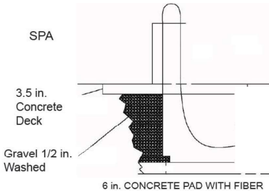
Figure 9. Excavation Cross Section
