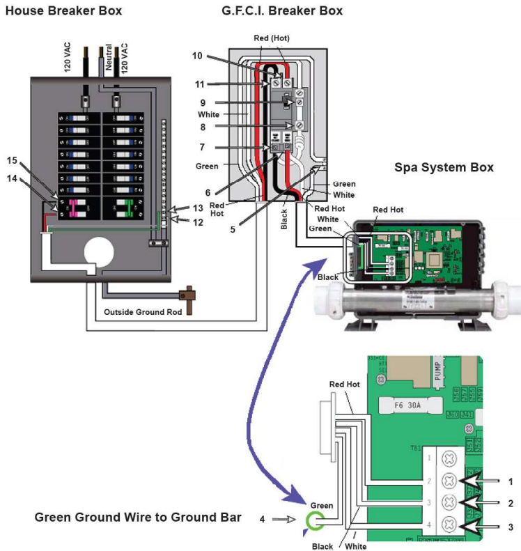
Figure 1. GFCI Wiring Schematic for 60 Hz Systems
