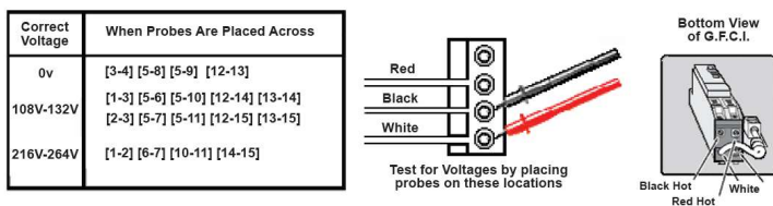
Figure 2. Proper Voltage Readings Across Terminals on House Breaker Box, Swim Spa and Exercise Pool System Box and GFCI
