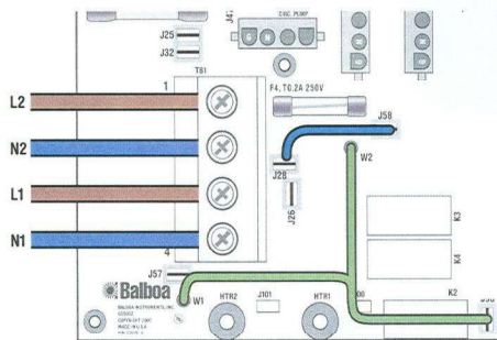
Figure 5. Two Phase Power – TN and TT Electrical Systems 2 x 16 A, 5 Wires (2 Lines + 2 Neutrals + 1 Protective Earth)
