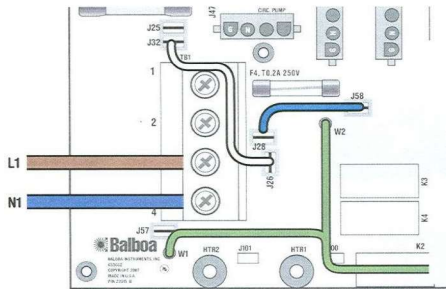
Figure 4. Single Phase Power – TN and TT Electrical Systems 1 X 16 A or 1 X 32 A, 3 Wires (1 Line + 1 Neutral + 1 Protective Earth (Ground))
