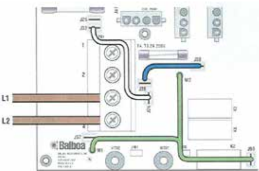
3 Phase Service, IT Electrical System (No Neutral)
