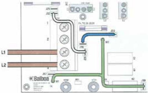
Single Service, IT Electrical System (No Neutral)
