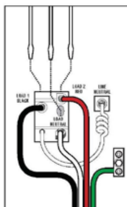
End View of Square D GFCI Breaker and Load Neutral Connection
