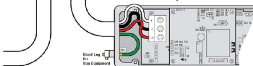
Main Electrical Connections In BP1500 System
