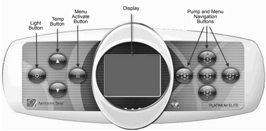
TOPSIDE CONTROLLER
