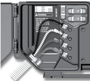
For 240 VAC (4 wires)
